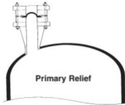
Figure 5. Bursting Disk
